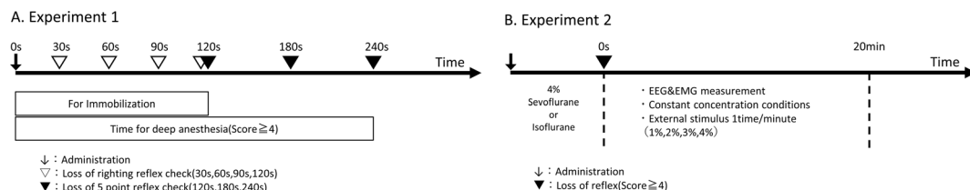
Fig. 1. Experimental design. (A) Experiment 1 was performed to investigate the effects of different concentrations of isoflurane or sevoflurane on the time of loss of the righting reflex after the introduction to anesthesia (checked at 30, 60, 90 and 120 s; n=18 for each concentration of both anesthetic drugs) and of loss of five-point reflex after deep anesthesia (checked at 120, 180, and 240 s; n=6 at each time point for each concentration of both anesthetic drugs). (B) Experiment 2 was performed to evaluate the effects of different concentrations of isoflurane or sevoflurane on the maintenance of deep anesthesia for 20 min based on EEG patterns, with an external stimulus given every minute. EEG, electroencephalography; EMG, electromyography.
