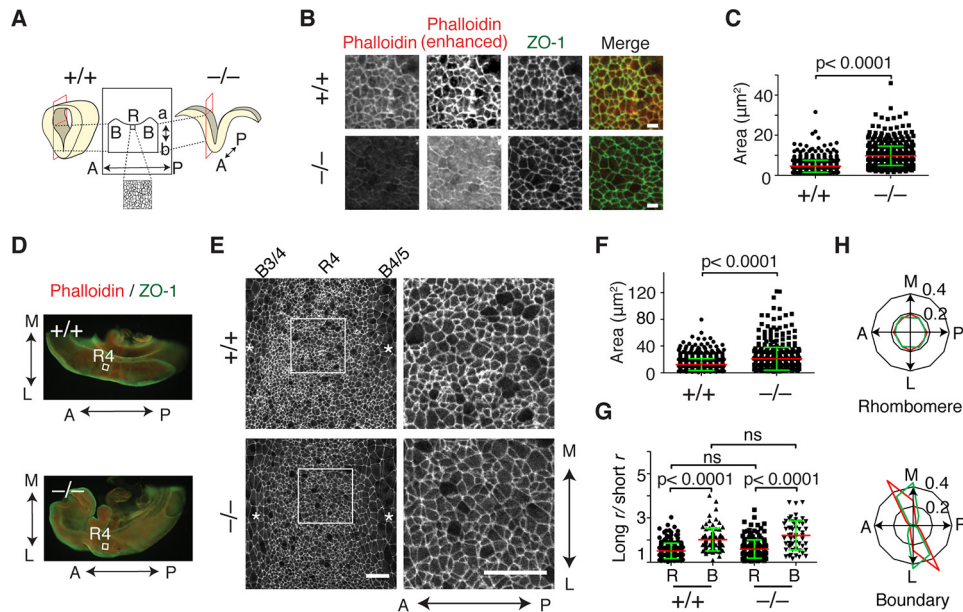
Figure 7. Apical constriction in the lateral neural plate of Fhod3 -/- embryos. A, schematic representation of the orientation of sagittal sections tangential to the apical plane used in B (B, boundary; R, rhombomere; a, apical; b, basal; A, anterior; P, posterior). B, apical view of the lateral neural plate at the level of rhombomere 4 in the hindbrain of Fhod3 +/+ (+/+) and Fhod3 -/- (-/-) embryos at E9.5. Sections were subjected to immunofluorescence staining for ZO-1 (green) and phalloidin staining for F-actin (red). Scale bars, 5 μm. C, quantification of apical cell surface area of sagittal sections. The apical surface area was estimated by ZO-1 staining of sections prepared from Fhod3 +/+ (n = 630 cells from 4 embryos) and Fhod3 -/- embryos (n = 758 cells from 4 embryos) shown in A. D, whole-mount staining of embryo halves. E9.5 embryos bisected at the midline were subjected to immunofluorescence staining for phalloidin (red) and ZO-1 (green). R4, rhombomere 4. E, apical view of whole-mount staining of ZO-1 at rhombomere 4 in the hindbrain from Fhod3 +/+ and Fhod3 -/- embryos at E9.5. Asterisks indicate inter-rhombomere boundaries. A↔P, anterior to posterior; M↔L medial to lateral. Scale bars, 25 μm. F, quantification of apical cell surface area of whole-mount embryos. The apical surface area was estimated by ZO-1 staining of whole-mount Fhod3 +/+ (n = 844 cells from 3 embryos) and Fhod3 -/- embryos (n = 532 cells from 3 embryos) shown in E. G, the anisotropy of the apical junction pattern. Cell outlines defined by ZO-1 staining shown in E were fitted to an elliptical shape, estimated by the ratio of the long to short radius (r) (rhombomere of Fhod3 +/+ , n = 224 cells from 3 embryos; boundary of Fhod3 +/+ , n = 88 cells from 3 embryos; rhombomere of Fhod3 -/- , n = 178 cells from 3 embryos; boundary of Fhod3 -/- , n = 55 cells from 3 embryos). For details, see "Experimental procedures." R, rhombomere; B, boundary; ns, not significant. Data are shown as mean (red line) ± S.D. (green lines). H, polar plots representing orientation of long-axis angles of cell outlines defined by ZO-1 staining shown in E. (red, Fhod3 +/+ ; green, Fhod3 -/- ). A↔P, anterior to posterior; M↔L medial to lateral.
