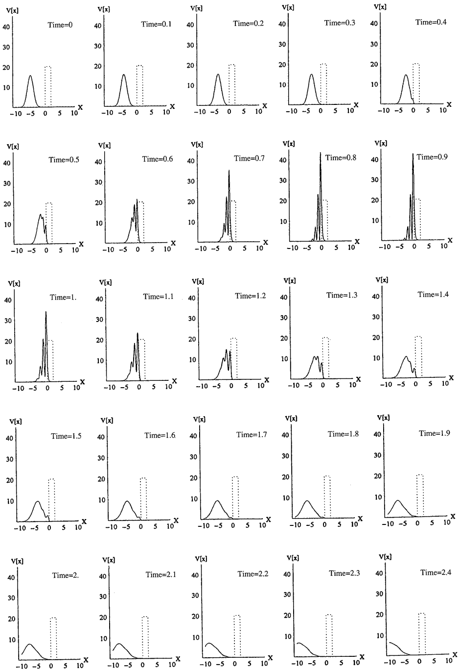
図9 Simulation④ ( E_0=10, V_0=20, a=2 )
