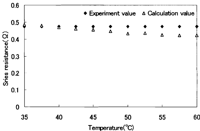
Fig.7 Series resistance on variable temperature.
