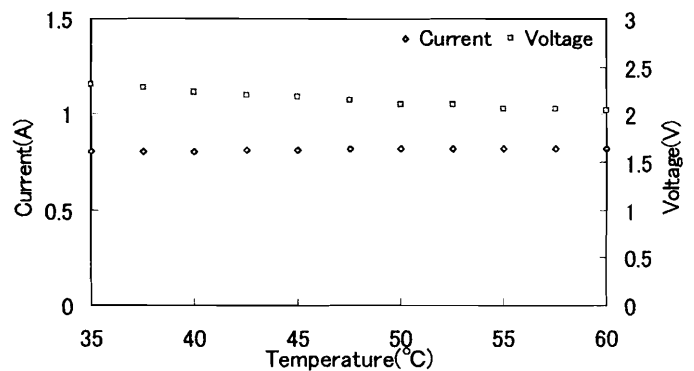
Fig.8 Open circuit voltage and short circuit current on measurement of series resistance.
