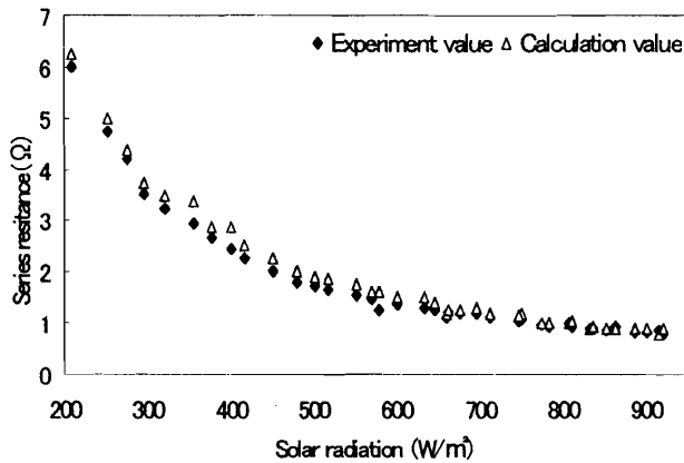
Fig.5 Series resistance on variable solar radiation.
